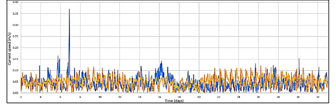
Figure 9. S Near-surface current speed magnitudes at the Loch Hourn salmon farm for the period 1 st -30 th December 2018. Blue lines are Mowi measured data and orange lines with symbols are the TELEMAC-3D predictions.
